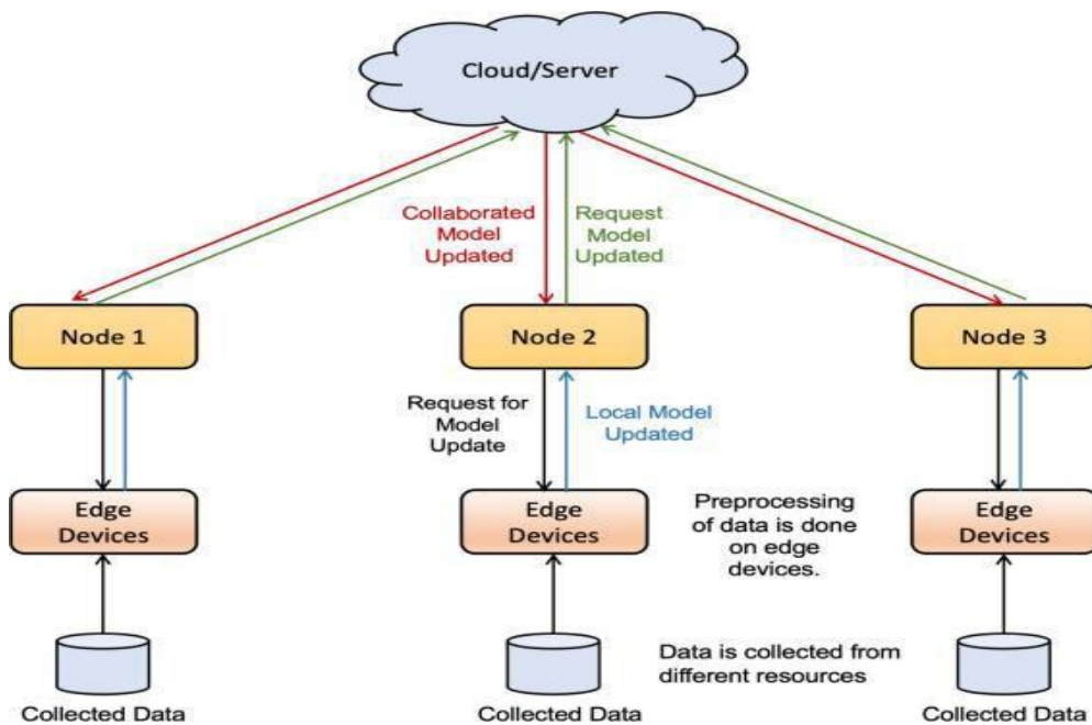
Figure: Federated Learning Architecture for Edge–Cloud Collaborative Model Updates
