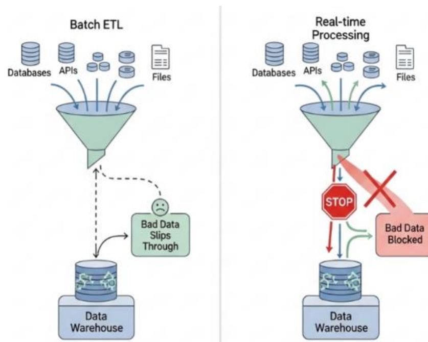
Fig 1: Real-Time Data Quality Monitoring
