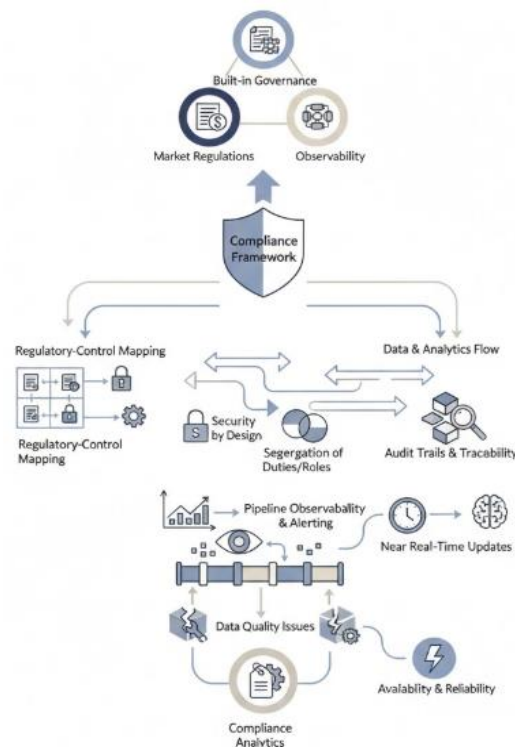
Fig 3: Integrated Governance by Design: A Multi-Layered Observability and Compliance Framework for High-Frequency Market Data Ecosystems
