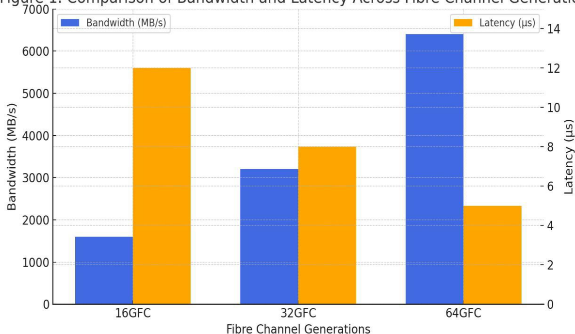
Figure 1. Comparison of Bandwidth and Latency Across Fibre Channel Generations
